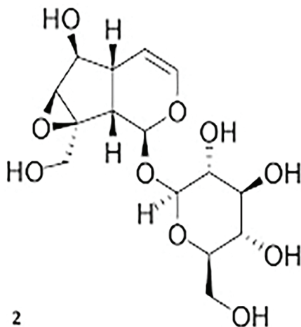
Figure 2. Catalpol, one of the iridoid glycoside molecules present in White Turtlehead; the ring structure to the lower right is glucose, the rest of the molecule is an example of an iridoid monoterpene. (Wikipedia)
